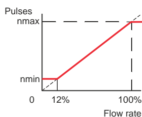
Scaled pulses
