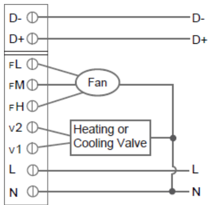
Fig. 3. Honeywell Home VC6013/VN6013 Wiring
